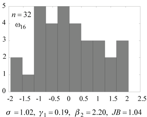
Fig. 4. Empirical distributions for n = 32
