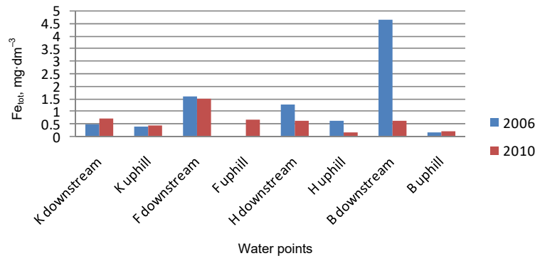
Fig. 11. Variation of the total iron ( \text{Fe}_{\text{tot}} ) concentration (2006–2010); water points as at Fig. 4; source: own study
