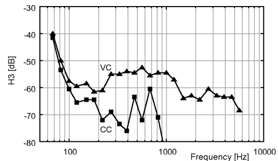
Fig. 18. Full-range driver 3rd harmonic distortion; level 2.83 Vrms.
