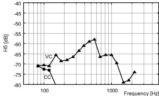
Fig. 16. Midrange driver #1 5th harmonic distortion; level 2.83 Vrms.
