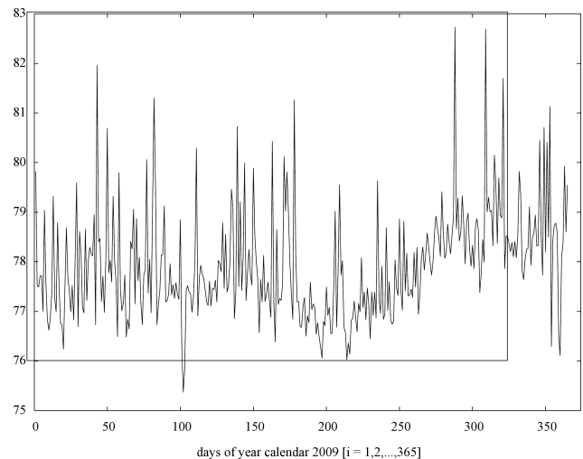
Fig. 1. Variability of L_{DEN} in the year 2009.
