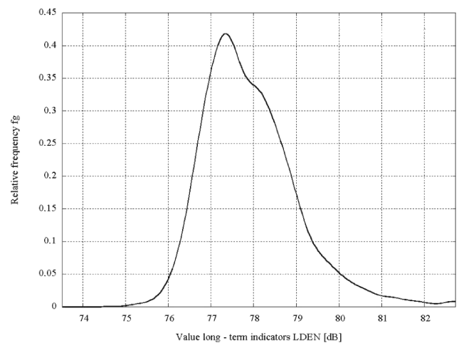
Fig. 2. Density probability distribution function of sound levels L_{DEN} .
