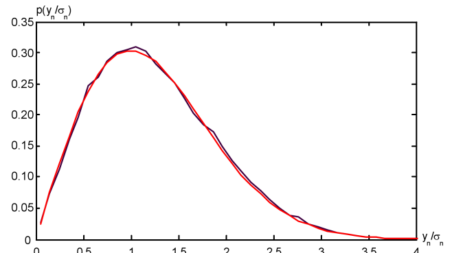
Fig. 9. Distribution of noise probability density at envelope detector output (theoretical – red line, simulation – black line) ( T = 10 s, f_0 = 10 kHz, B = 2 kHz, B_i = 0.4 kHz, SPL = 50 dB, M_i = 10 ).
