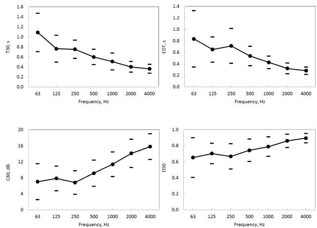
Fig. 18. Corridor – average values of the acoustic parameters; STI = 0.78.
