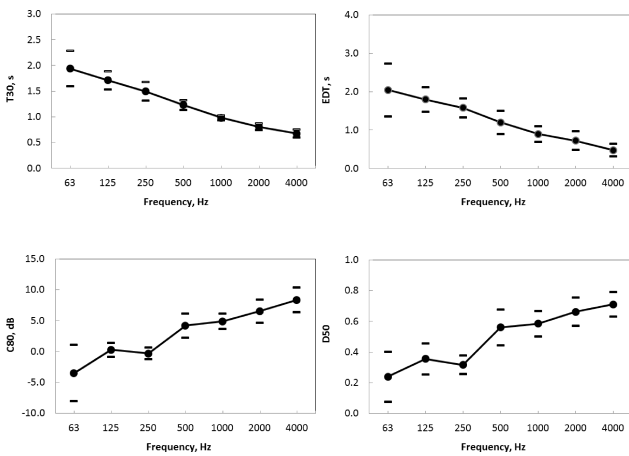
Fig. 6. First level – average values of the acoustic parameters, STI = 0.66.
