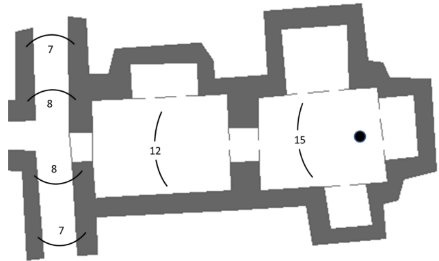
Fig. 23. C_{80} average spatial distribution.
