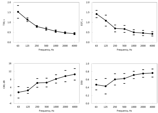
Fig. 17. Double cubicle – average values of the acoustic parameters; STI = 0.73.
