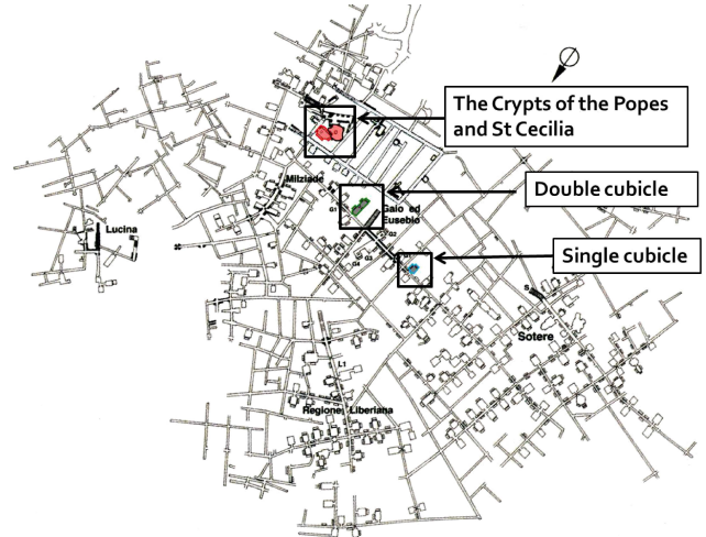
Fig. 12. Plant of the catacombs of “San Callisto”, with the places in which the acoustic measurements were carried out.
