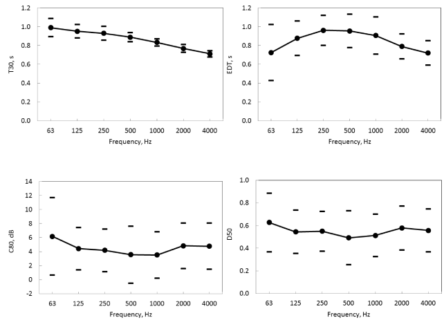
Fig. 16. Crypt of St Cecilia – average values of the acoustic parameters; STI = 0.64.
