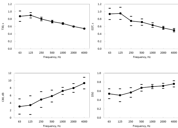
Fig. 15. Crypt of Popes – average values of the acoustic parameters; STI = 0.71.
