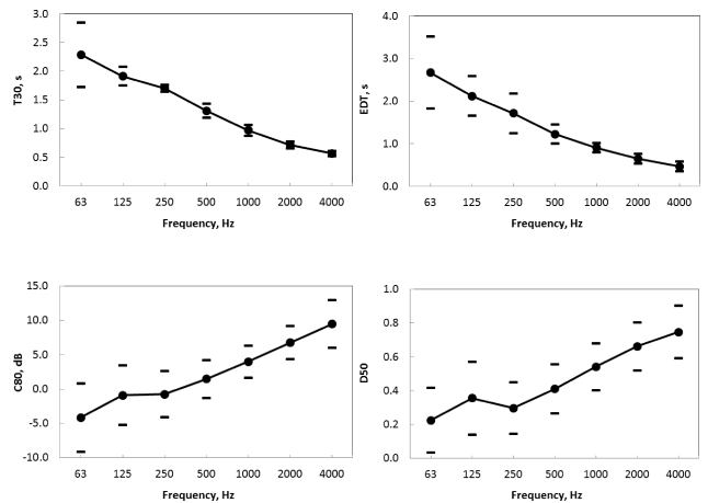
Fig. 9. Second level – average values of the acoustic parameters, STI = 0.60.
