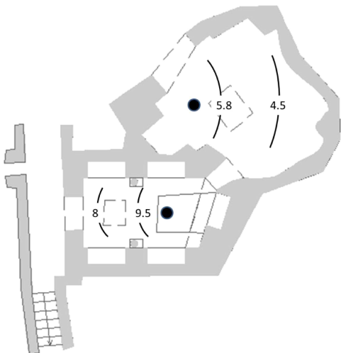
Fig. 21. C_{80} average spatial distribution.
