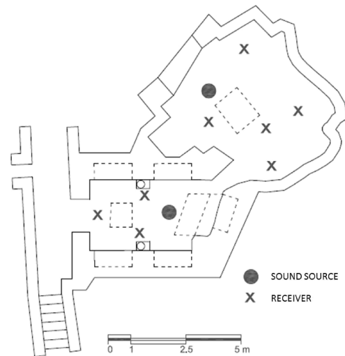
Fig. 13. Plant of the Crypts of Popes and Crypts of St. Cecilia.
