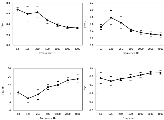
Fig. 19. Single cubicle – average values of the acoustic parameters; STI = 0.78.
