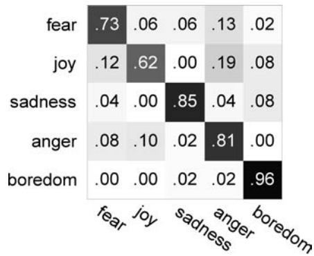
Fig. 3. Confusion matrix for the SPLSR method.
