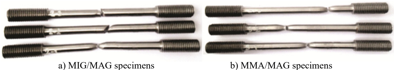
Fig. 12. Specimens with welded joint after testing
