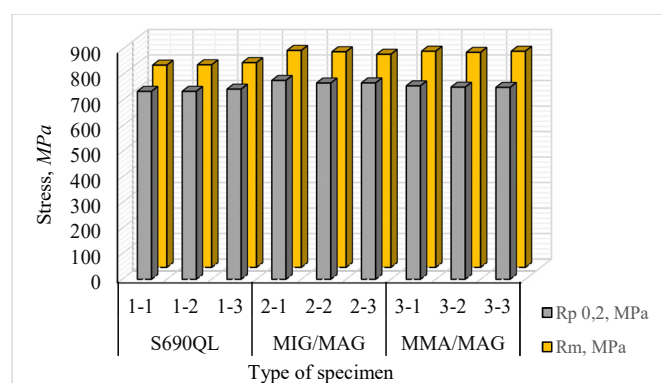
Fig. 10. Basic mechanical properties of specimens
