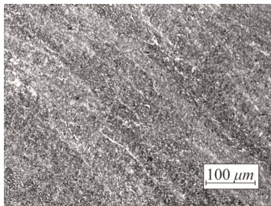
Fig. 7. Microstructure of weld metal at face of welded joint, magnification 200 times
