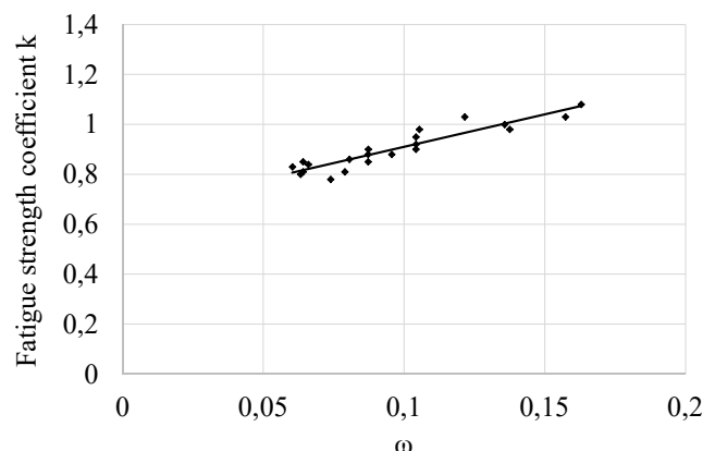
Fig. 2. Fatigue strength coefficient k of hardened steel tempered at 300°C subject to the quotient of the diameter of impurities and the spacing between impurities \omega
