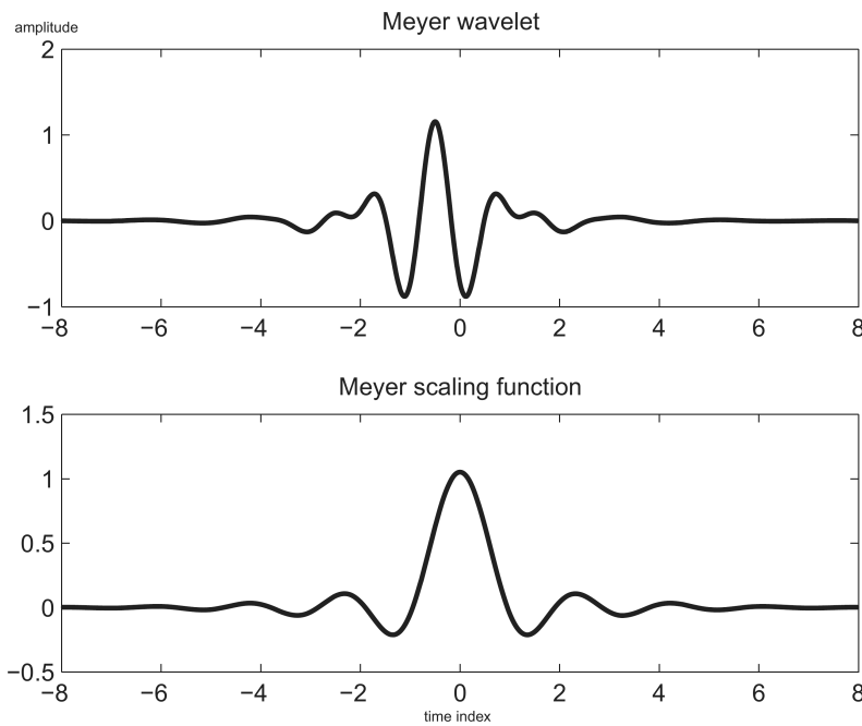
Fig. 2. The discrete Meyer wavelet \psi(n) and its scale function \phi(n) .
