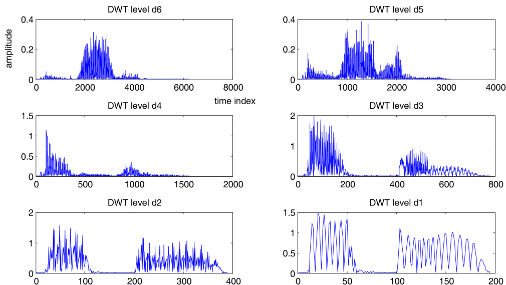
Fig. 3. Subband amplitude DWT spectra of the Polish word ‘osiem’ (Eng. eight). The number of samples depends on a resolution level.
