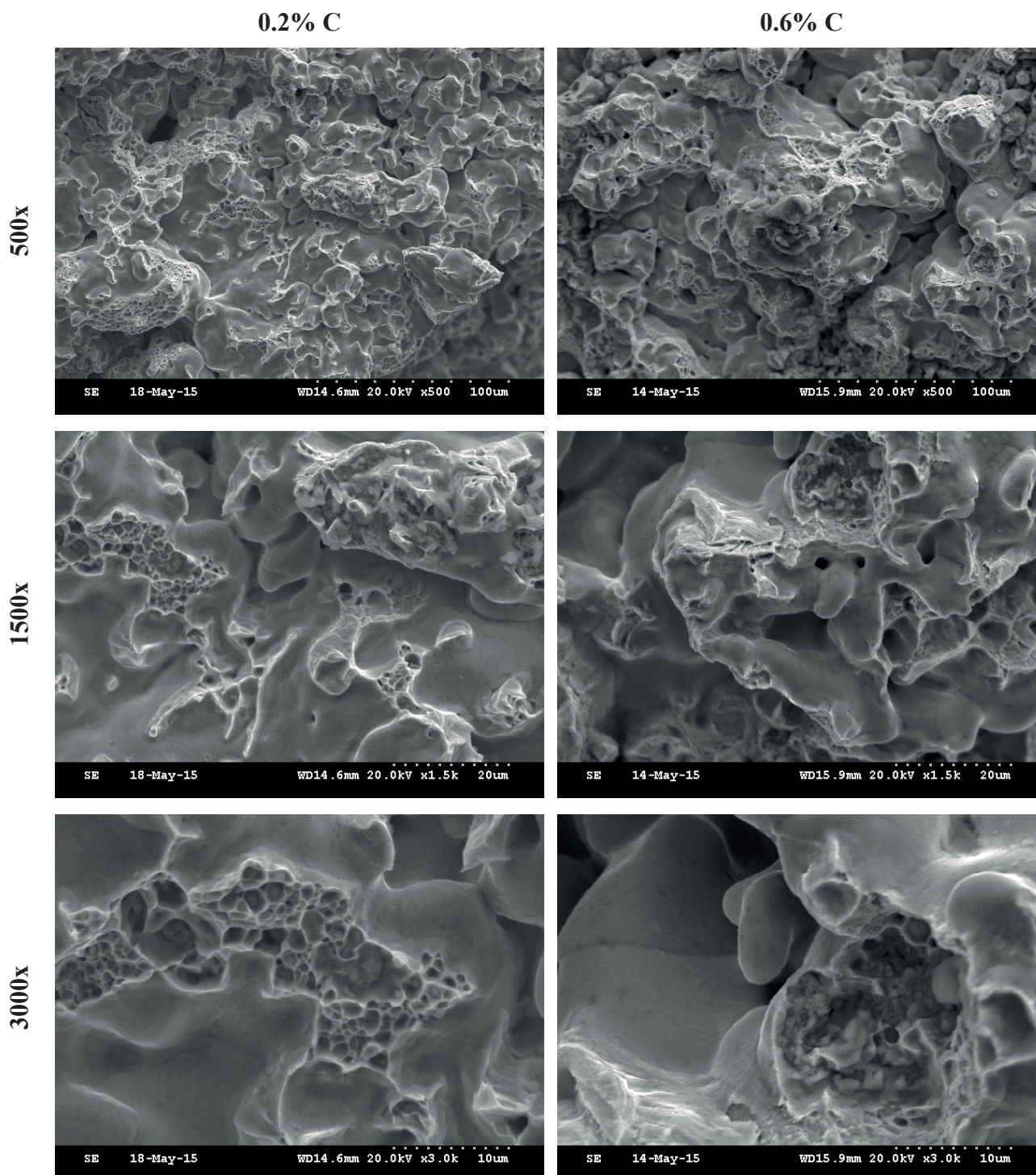
Fig. 2. The fracture of PM steels based on pre-alloyed Astaloy CrA powder, sintered at 1120°C (SEM)
