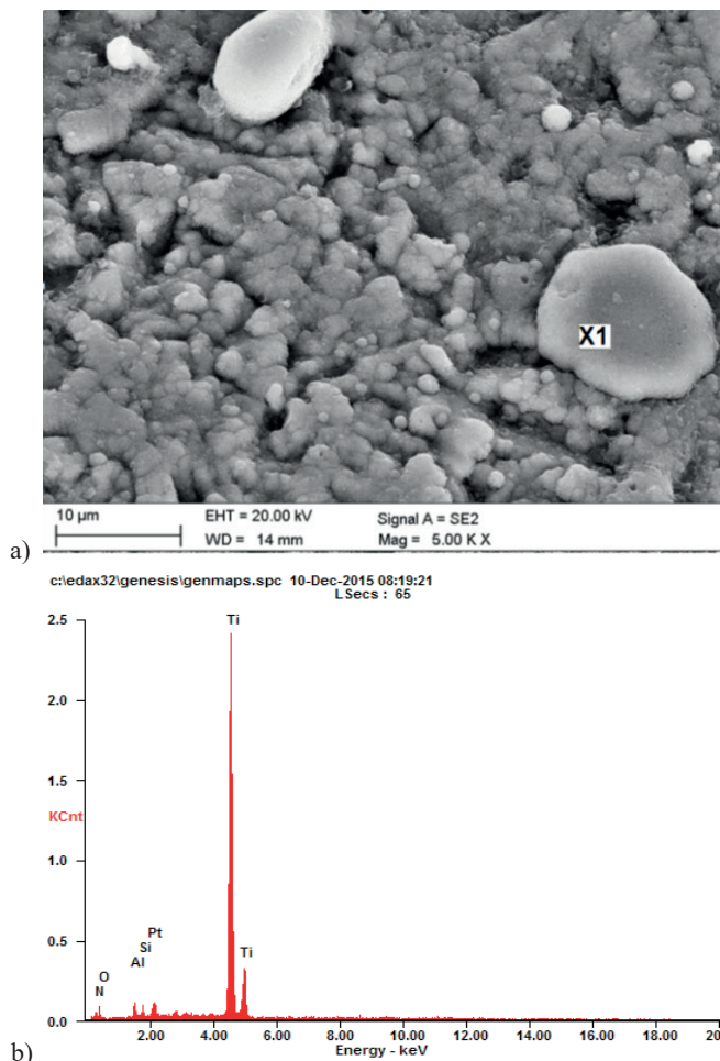
Fig. 2. a) Surface topography and b) the X-ray energy dispersive plots from the microzones X1 of the Ti(C,N) coating surface, deposited onto the Si 3 N 4 nitride ceramics
