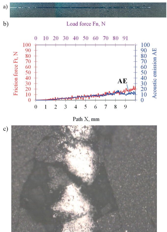
Fig. 8 (a) Trace of the scratch test; (b) diagram of the dependence of friction force ( F_t ) and Acoustic Emission (AE) on the load and (c) failure by 30 N load – for the Ti(C,N) coating deposited on Si 3 N 4 nitride ceramics (magnification 200x)
