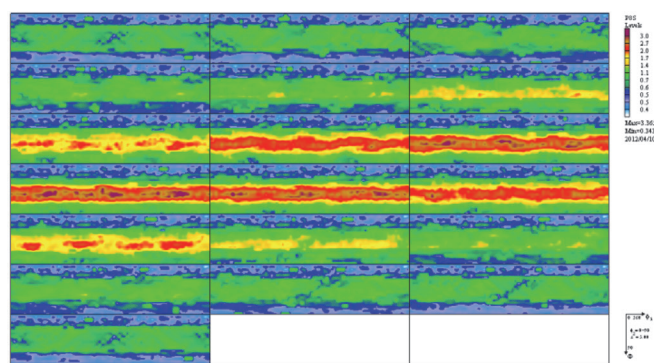
Fig. 5. Orientation distribution function of Ti(C,N) coating obtained in the PVD process on sialon ceramics substrate: a) cross section after φ 2 (for the following φ 2 values: 0, 5, 0...90°)
