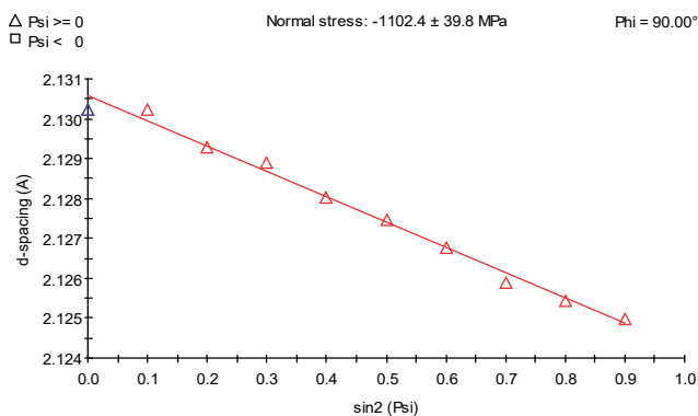
Fig. 6. Variations in the interplanar distance value of d reflex (200) of the Ti(C,N) coating obtained in PVD process on the substrate made of s ceramics in the function of \sin^2\psi (measurement of stresses with the \sin^2\psi method) - measurement along the main cutting edge
