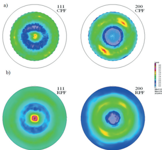
Fig. 4. Pole figures (111), (200) of Ti(C,N) coating obtained in the PVD process on sialon ceramics substrate: a) experimental, b) calculated from ODF
