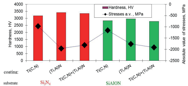
Fig. 7. Comparison of microhardness and residual stresses of investigated coatings deposited on the nitride and sialon ceramics
