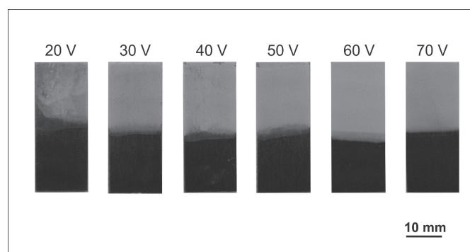
Fig. 3. Macroscopic images of as-deposited \text{SiO}_2/\text{HAp} coatings on Cp-Ti1 at different voltage and constant deposition time equal to 60 seconds
