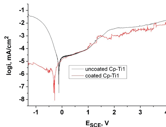
Fig. 9. Anodic polarization curves for Cp-Ti1 and \text{SiO}_2/\text{HAp} coating on Cp-Ti1 in Ringer's solution at 37^\circ\text{C} and 1 mV/s
