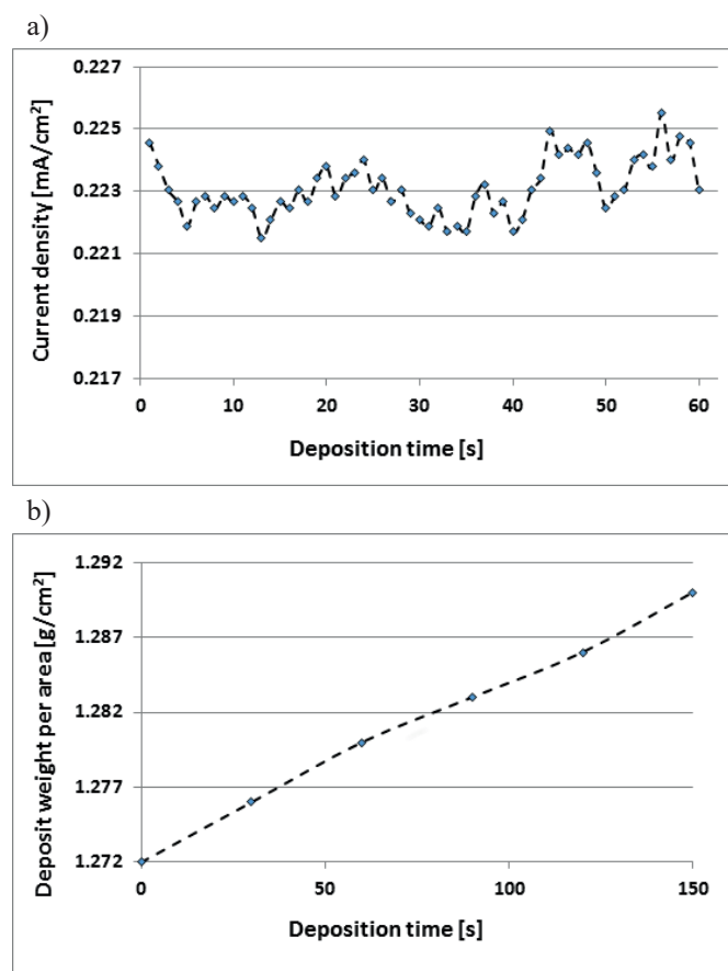
Fig. 4. Typical dependence of deposition time on current density during EPD (a) and weight change of as-deposited coatings at constant voltage of 60 V for different deposition time (b)
