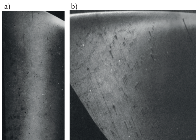
Fig. 4. Silicon. Entrance surface is (001). Skew asymmetric (331) reflection, \text{CoK}_\alpha -radiation: a) \phi_0=3^\circ , L_{ext}=3.4 \mu\text{m} ; b) \phi_0=1^\circ , L_{ext}=1.39 \mu\text{m}
