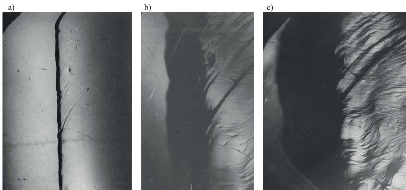
Fig.5. Surface relief of InSb/InSb homoepitaxial systems grown in hydrogen atmosphere at temperature 440^\circ\text{C} [12, 13]. Entrance surface is (111). (511) reflection, \text{CuK}_\alpha -radiation: a) \phi_0=3^\circ , L_{ext}=2.89 \mu\text{m} ; b) \phi_0=1^\circ35' , L_{ext}=1.25 \mu\text{m} ; c) \phi_0=0^\circ41' , L_{ext}=0.95 \mu\text{m}
