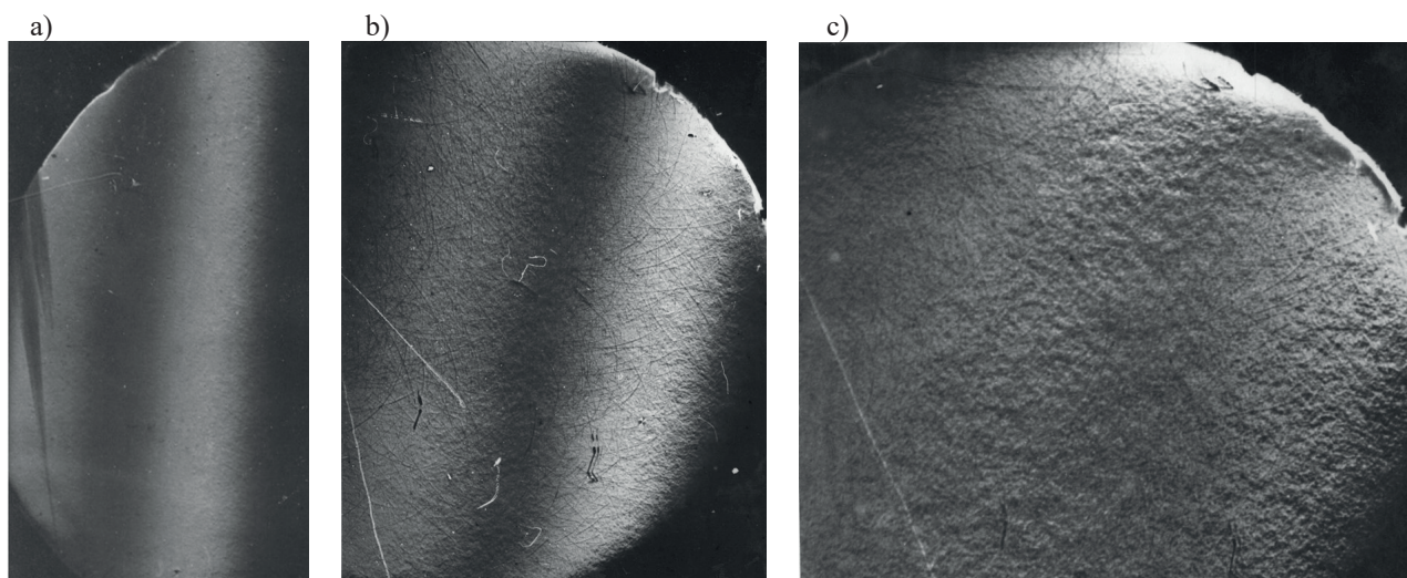
Fig. 3. Subsurface distortions in CdTe crystals after standard mechanochemical treatment of surface [10]. Entrance surface is (111). (511) reflection, \text{CuK}_\alpha -radiation: a) \phi_0=29^\circ , L_{ext}=5.42 \mu\text{m} ; b) \phi_0=1^\circ35' , L_{ext}=1.89 \mu\text{m} ; c), \phi_0=0^\circ33' , L_{ext}=1.26 \mu\text{m}
