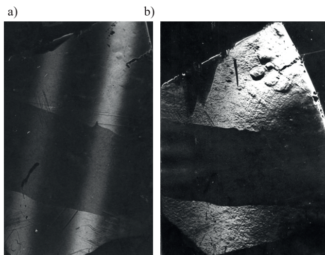
Fig. 8. Morphology and structural change of the surface of \text{Cd}_{1-x}\text{Hg}_x\text{Te}/\text{CdTe} epitaxial layers after implantation by As ions ( E=100 keV, D_1=10^{15} ion/cm 2 ) [12]. Entrance surface is (111). (511) reflection, \text{CuK}_\alpha -radiation: a) \phi_0=3^\circ , L_{\text{ext}}=1.44\mu\text{m} , b) \phi_0=0^\circ 41' , L_{\text{ext}}=0.75\mu\text{m}
