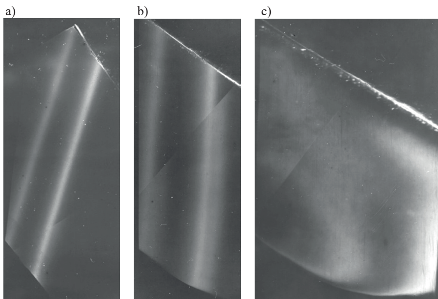
Fig. 7. Silicon. Entrance surface is (001). Skew asymmetric (331) reflection, \text{CoK}_\alpha -radiation. The energy is E=180 keV, and dose of implantation of phosphorus ions is Q=10^{15} ion/cm 2 : a) L_{\text{ext}}=0.94\mu\text{m} , b) 0.65\mu\text{m} , c) 0.25\mu\text{m}
