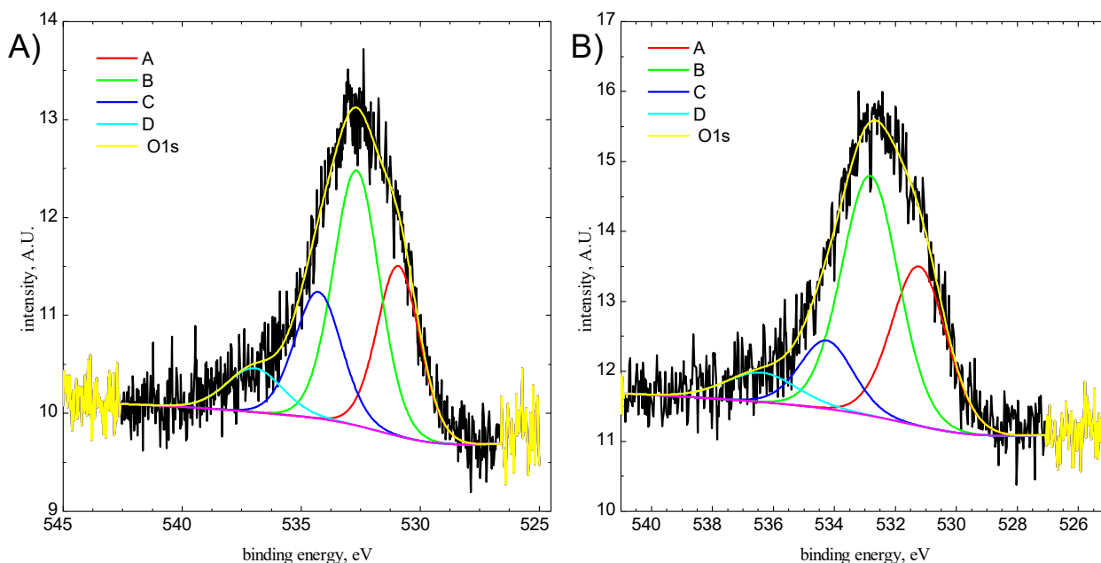
Fig. 3. High resolution of XPS spectra of the O1s core excitation A) before adsorption, and B) after adsorption
