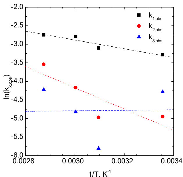
Fig. 7. Influence of temperature on k_{x,obs}
