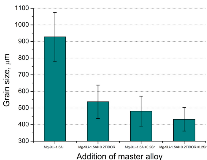
Fig. 6. Grain sizes of Mg-9Li-1.5Al cast alloy with additions of TiBor and AlSr10
