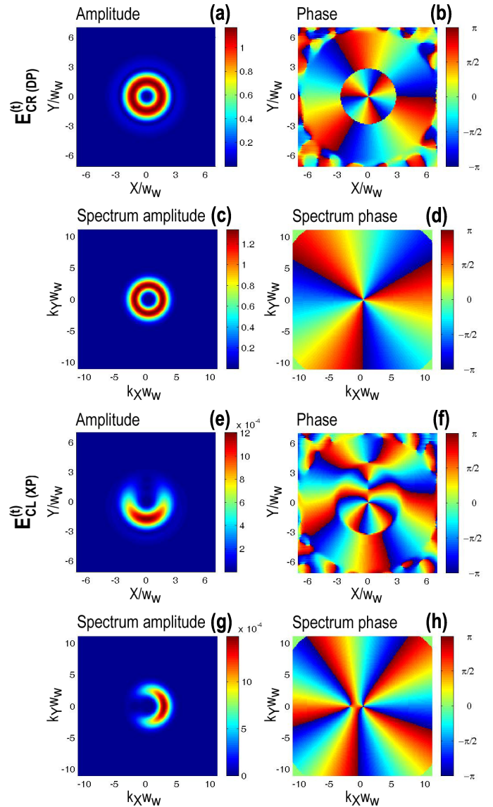
Fig. 7 (colour online). Transmitted components of the CR incident ELG beam, p = 1, l = 3 (see Fig. 3) in the case of the “significant” incidence, \Theta_i = \Theta_S \cong 2^\circ for k_i w_w = 10 \cdot 2\pi . The two first (second) rows show the DP (XP) component of the transmitted beam. The first and second column are respectively the amplitude and phase decompositions in the spatial and spectral domains. The third and fourth rows show the amplitude and phase of spectral components. Values on the axis of abscissa are shown with reference to the global shift k_i w_w \sin \theta_i . (a)–(d) the CR (DP) component of transmitted beam, (e)–(h) the CL (XP) component of the transmitted beam. The amplitude of the total transmitted field (is not shown here) is similar to the DP component.
