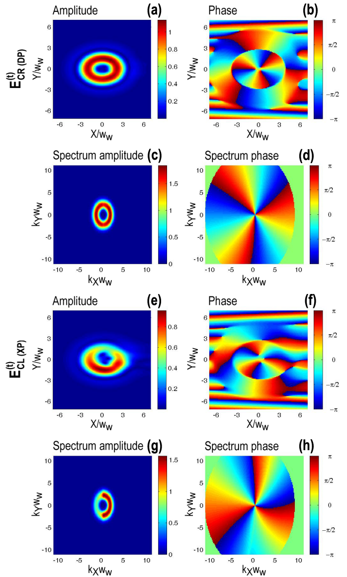
Fig. 9 (colour online). Transmitted components of the CR incident ELG beam p = 1, l = 3, k_i w_w = 10 \cdot 2\pi (see Fig. 3) in the case of the critical incidence. The first two (second) rows show the DP ( XP ) component of the transmitted beam. The first and second column are respectively the amplitude and phase decompositions in the spatial and spectral domains. The third and fourth rows show the amplitude and phase of spectral components. Values on the axis of abscissa are shown with reference to the global shift k_i w_w \sin \theta_i . (a)–(d) the CR ( DP ) component of the transmitted beam, (e)–(h) the CL ( XP ) component of the transmitted beam. The amplitude of the total transmitted field (is not shown here) is similar to the DP component but influence of the presence of half-moon in the XP component is also visible.
