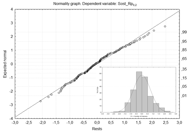
Fig. 3. Verification of the agreement of the distribution of the Sost Rp0.2 variable residue with the normal distribution
