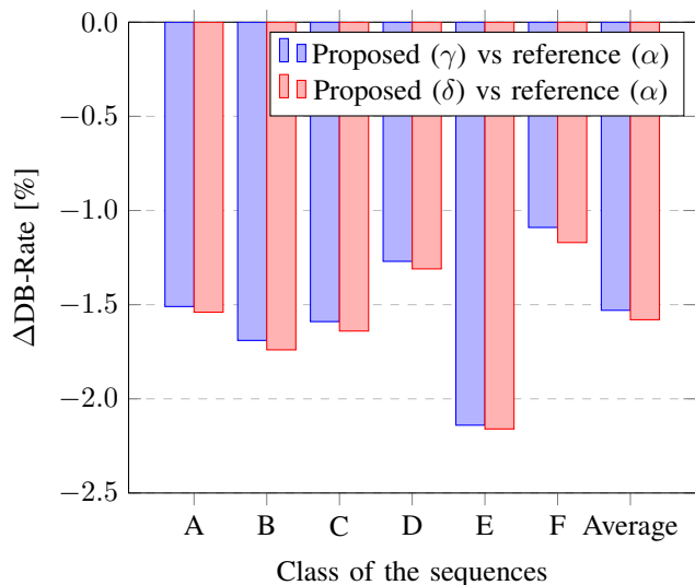
Fig. 12. Summary of Bjøntegaard deltas [29] of the proposed (\gamma) versus original sequence encoding (\alpha) and the proposed with motion vectors reestimation (\delta) versus original sequence encoding (\alpha) . Negative values indicate bitrate reductions.
