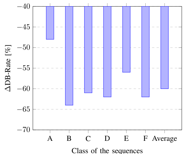
Fig. 13. Summary of Bjøntegaard deltas [29] of the denoised (\beta) sequence encoding versus original sequence encoding (\alpha) . Negative values indicate bitrate reductions.
