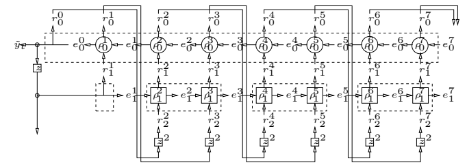
Fig. 11. Modeling p -invariant filter ( p = 1 ).
