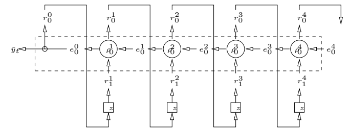
Fig. 10. Modeling p -invariant filter ( p = 0 ).
