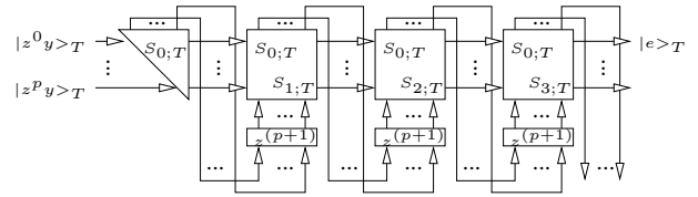
Fig. 4. Block-orthogonalization of the basis of the space S_T ( N = 3 ) – the p -stationary case: 'triangle' - auto-orthogonalization of the basis of S_{0;T} ; 'squares' - mutual orthogonalization of the bases of S_{0;T} and S_{n;T} ( n = 1, 2, 3 ).
