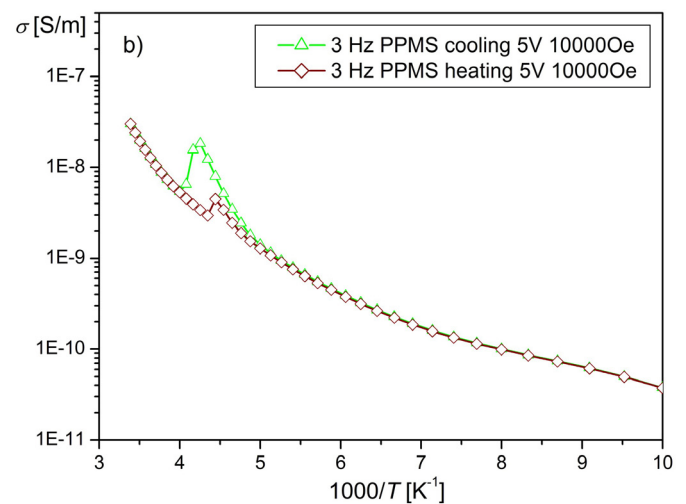
Fig. 5. Dependencies \ln\sigma(1000/T) depending on measuring cycle (heating, cooling) and constant magnetic field for the PFN ceramics
