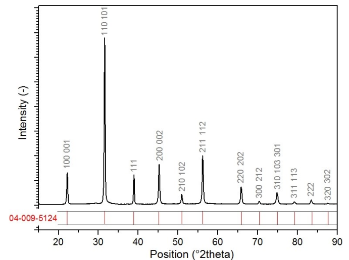
Fig. 1. X-ray diffraction pattern for the investigated PFN ceramics
