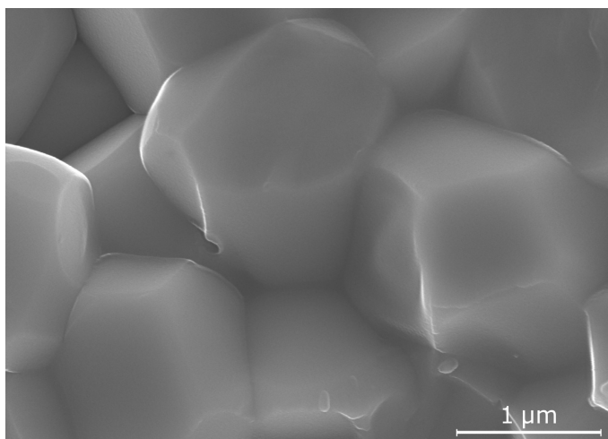
Fig. 2. SEM microstructure of the PFN ceramics
