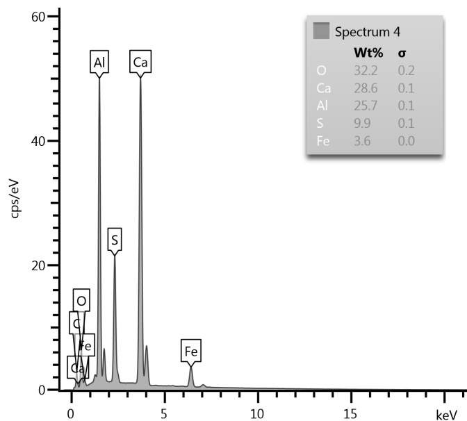
Fig. 11. X-ray microanalysis of a fatigue centre formed during a test conducted by the resonance method of a specimen of 15CrNi6 steel
