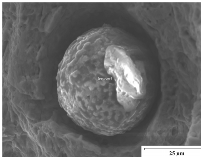
Fig. 6. A SEM image of a non-metallic inclusion revealed under a carburized layer for 15CrNi6 steel following low pressure carburizing and oil quenching
