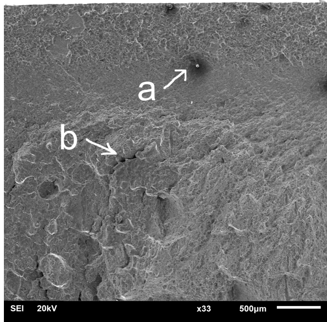
Fig. 8. A SEM image of a fatigue fracture for 15CrNi6 steel following low pressure carburizing and oil quenching; a. inclusion under the hardened surface with: a. formed “pocket”, b. longitudinal cracks of the specimen
