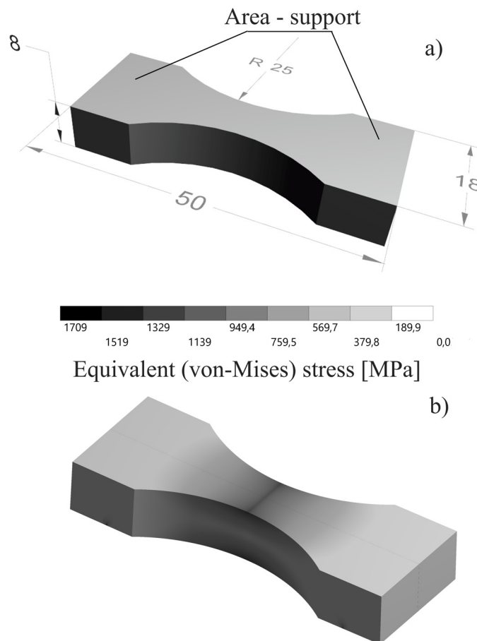
Fig. 2. a. The shape of the specimen designed for fatigue testing, b. distribution of von Mises reduced stress in a specimen for bending fatigue strength tests by the one-side three-point bending
