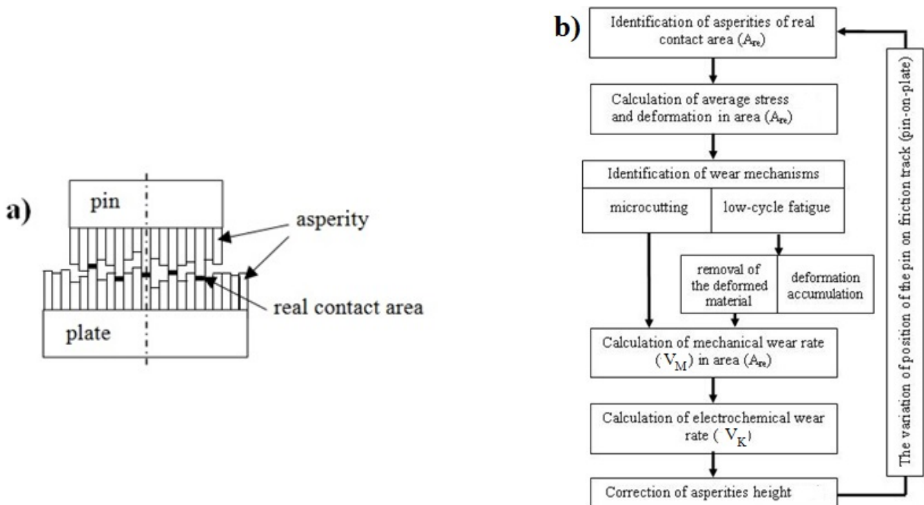
Fig. 2. Computational model: a) axial cross-section of the pin-on-plate combination, b) computational algorithm of tribocorrosion process in sliding pair
