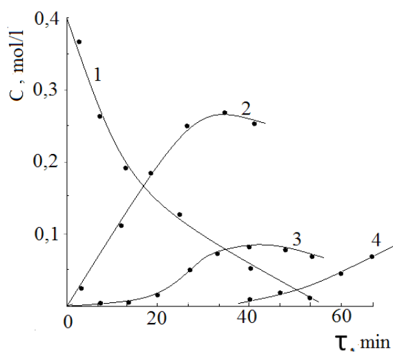
Fig. 1. Kinetics of oxidation of 3-acetylaminotoluene in acetic anhydride at 20°C in the presence of sulfuric acid manganese (II) acetate: 1- 3-acetylaminotoluene; 2- 3-acetylaminobenzylacetate; 3- 3-acetylaminobenzylidendiacetate; 4 - 3-acetylaminobenzoic acid; [ArCH_3]_0 = 0.4 ; [Mn(OAc)_2]_0 = 0.08 ; [H_2SO_4]_0 = 1.0 ; [O_3]_0 = 4.0 \cdot 10^{-4} mol/l; V_p = 0.01 l
