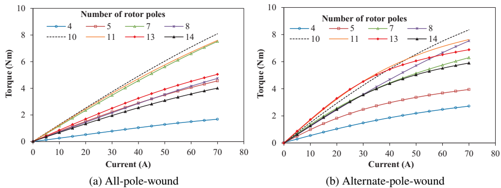
Fig. 7. Comparison of average torque against current, i_d = 0
