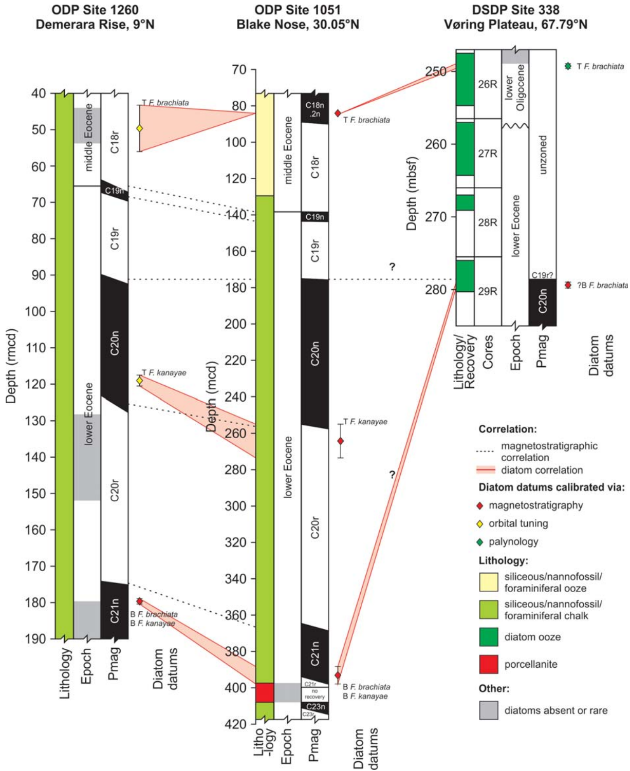
Text-fig. 9. Fence diagram showing the stratigraphic position of base (B) and top (T) for the stratigraphic ranges of Fenneria kanayae (Fenner) J. Witkowski, comb. nov. and Fenneria brachiata (Brightwell) J. Witkowski, comb. nov. at DSDP Site 338, and ODP Sites 1051 and 1260. Abbreviations: rmcd = revised metres composite depth; mcd = metres composite depth; mbsf = metres below sea floor; pmag = magnetostratigraphy. Site 1260 correlation based on data from: Erbacher et al. (2004), Suganuma and Ogg (2006), Renaudie et al. (2010), and Westerhold and Röhl (2013). Site 1051 correlation based on data from Norris et al. (1998b), Ogg and Bardot (2001), Edgar et al. (2010), and Luciani et al. (2016). Site 338 correlation based on data from Schrader and Fenner (1976), Dzinoridze et al. (1978, 1979) and Eldrett et al. (2004)
