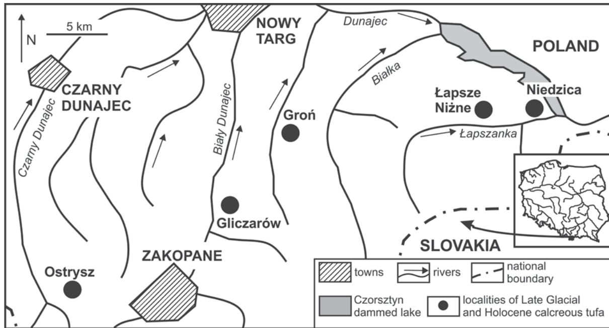
Text-fig. 1. Location of profiles of Late Glacial and Holocene calcreous tufa in Podhale Basin
