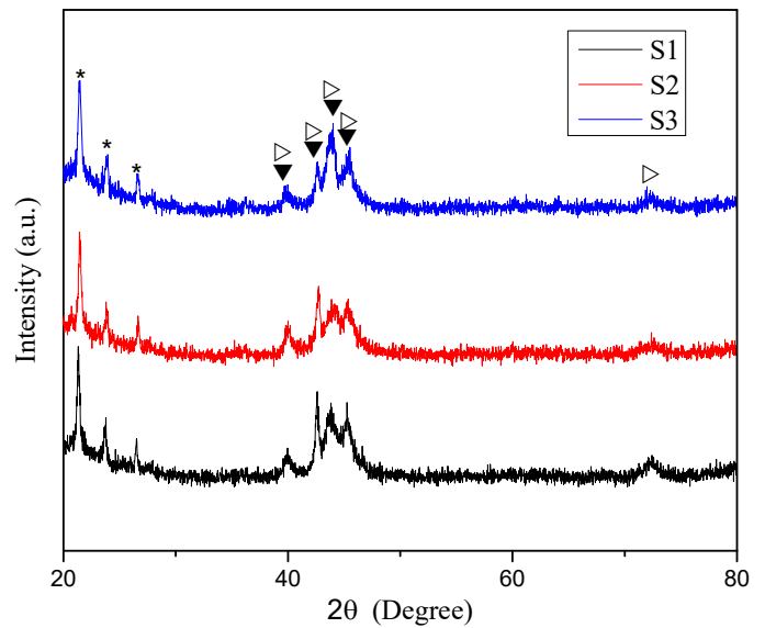
Fig. 1. X-ray diffractograms of Cu-Al-Cr shape memory alloy systems at room temperature (*: \text{Cu}_9\text{Al}_4 , ▷: \gamma_1' martensite phase, ▽: \beta_1' martensite phase)
