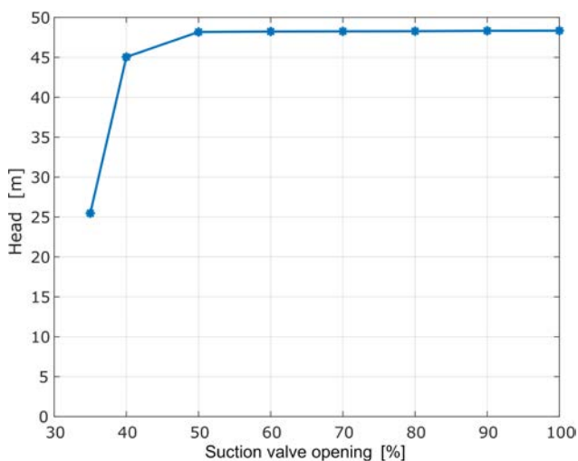
Fig. 5. Relation between head and different suction valve openings at 103 l/min.
