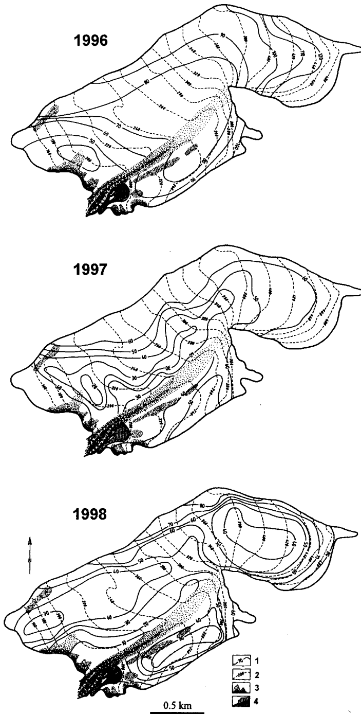
Fig. 3. Map of snow accumulation on the Waldemar Glacier in May 1996–1998. 1 – snow accumulation isolines (in cm w.e.), 2 – contour lines, 3 – median and surface moraine, 4 – ice-dam lake.
