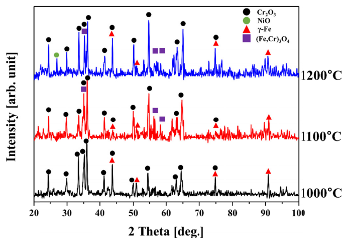
Fig. 4. XRD phase analysis results after high temperature oxidation tests of MIMed HK30 alloy
