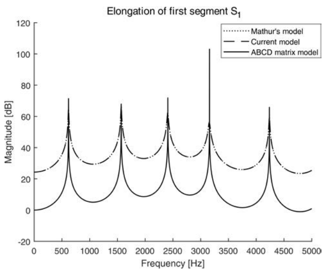
Fig. 8. Comparison of formant frequencies of the current model and Mathur's model with ABCD matrix model for the elongated segment S_1 .
