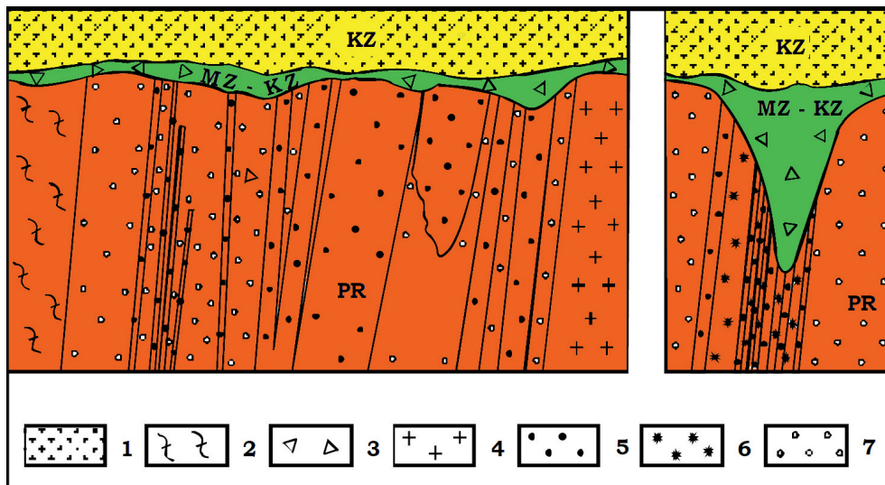
Fig. 2. Novopoltavka deposit (schematic geological section) (Mychajlov et al. 2007)
