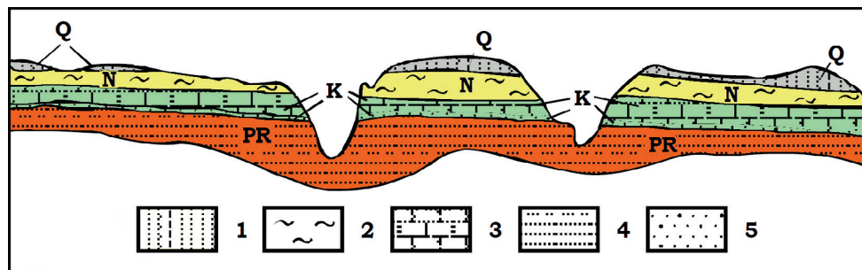
Fig. 3. Zhvan deposit (schematic geological section) (Mychajlov et al. 2007)
