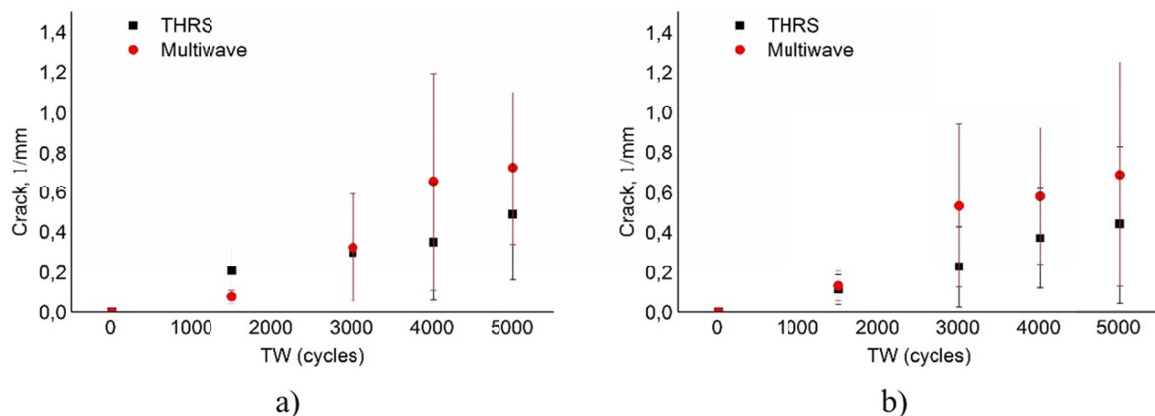
Fig. 6. Crack length versus cycle number a) -30/+110^\circ\text{C} thermal profile, b) -40/+125^\circ\text{C} thermal profile
