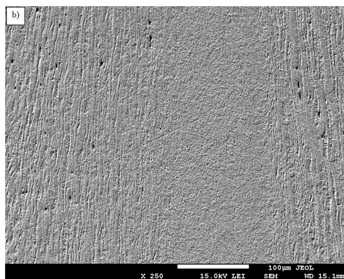
Fig. 9. SEM in the LEI mode of the transverse section of the friction welded joint sample, a) mag. \times 40 , b) mag. \times 250
