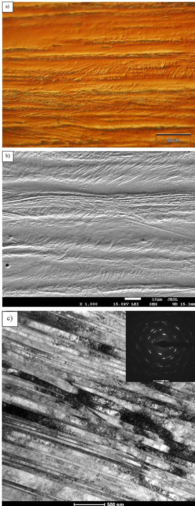
Fig. 4. Microstructure of 316L steel after one-pass hydrostatic extrusion, longitudinal cross-section: a) Optic micrograph (Olympus IX70) in Nomarski interference contrast (DIC), magnification \times 500 , b) SEM in the LEI mode of sample (scanning electron microscope JEOL JSM-7600F), c) Bright field TEM images with corresponding SAED patterns
