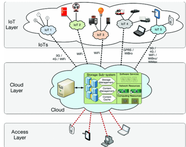
Fig. 1. The interactions within Cloud of Things
