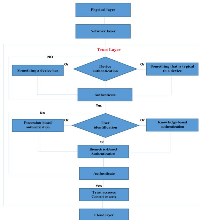
Fig.2. E-government trust framework for Cloud of Things
