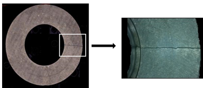
Fig. 5. Die with visible crack
