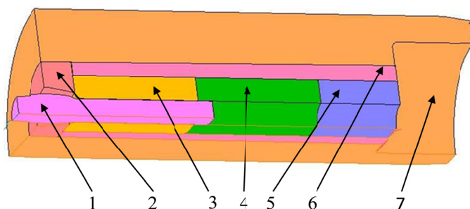
Fig. 4. Geometric model of the a tool systems with individual deformable bodies: 1 – screw, 2 – die, 3, 4, 5 – spacer sleeve, 6 – the centering tube blank, 7 – casing
