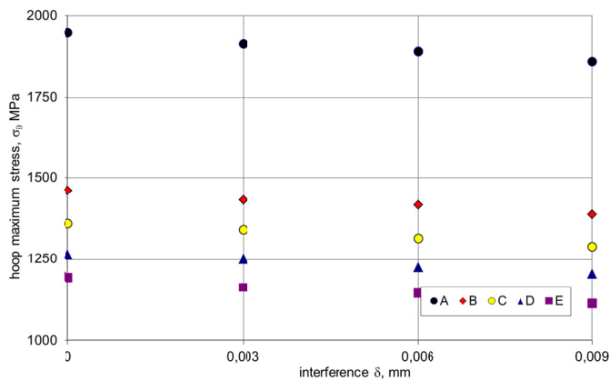
Fig. 10. The values of hoop maximum stress in the measurement points of tools during the forging of the screw head depending on the interference used
