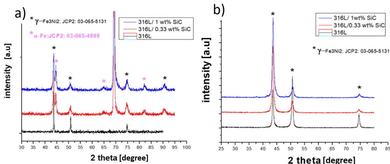
Fig. 6. XRD diffractograms of 316L /SiC a) the milled powder mixtures in comparison with the 316L powder, b) the sintered composites in comparison with the sintered 316L sample
