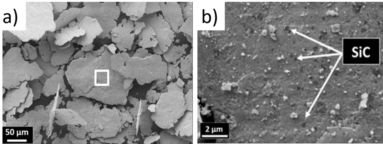
Fig. 2. SEM micrographs of the milled 316L/0.33 wt% SiC. a) milled powders, b) higher magnification of the selected area in Fig. 2a
