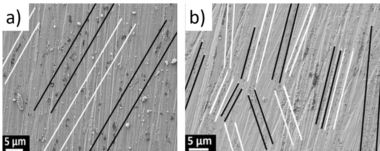
Fig. 7. SEM micrographs of the sintered composites. a) 316L/0.33wt % SiC, b) 316L/ 1wt % SiC
