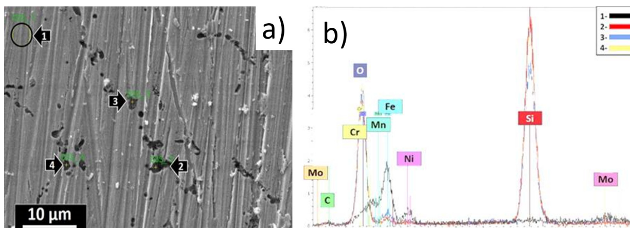
Fig. 8. SEM (a) and EDS (b) investigation of the 316L/0.33wt% SiC
