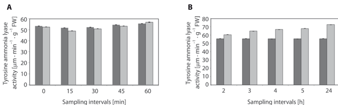
Fig. 8. Tyrosine ammonia lyase (TAL) activity in 8-week-old tomato plants in minutes (A) and hours (B) post inoculation; FW – fresh weight
