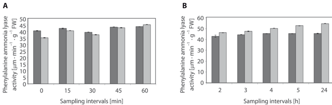
Fig. 7. Phenylalanine ammonia lyase activity (PAL) in 8-week-old tomato plants in minutes (A) and hours (B) post inoculation; FW – fresh weight
