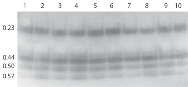
Fig. 5. Native PAGE of cytoplasmic polyphenol oxidase (PPO) PPO (sampling at 0–60 min): Lane 1 – control at 0 min; Lane 2 – Aspergillus niger treated at 0 min; L3 control at 15 min; L4 – treated at 15 min; L5 – control at 30 min; L6 – treated at 30 min; L7 – control at 45 min; L8 – treated at 45 min; L9 – control at 60 min; L10 – treated at 60 min. Numerical values represent the respective Rf value of each band
