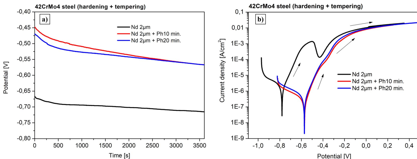
Fig. 4. A course of an open circuit potential a) and polarization curves b) determined after 1 hour of immersion in 0,5 M NaCl for samples of 42CrMo4 nitrated steel (nitrated layer 2 \mu\text{m} ) and after 10 min. and 20 min. of phosphating
