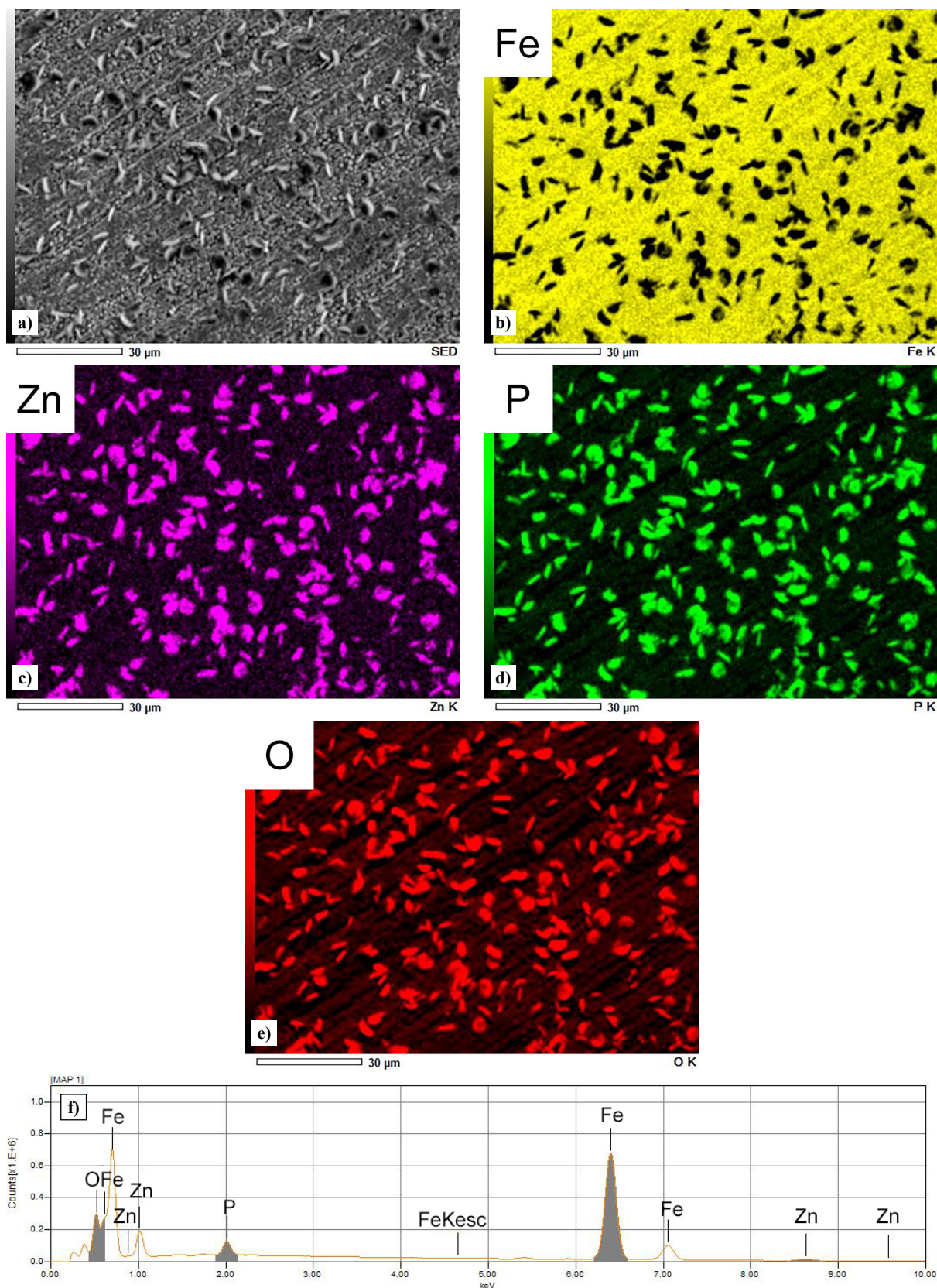
Fig. 3. SEM image (a) and EDS mapping of composition of Nd 16 \mu\text{m} sample after phosphating during 5 seconds: (b) the EDS mapping of element Fe, (c), (d) and (e) EDS mapping of elements Zn, P and O respectively, (f) EDS element analysis
