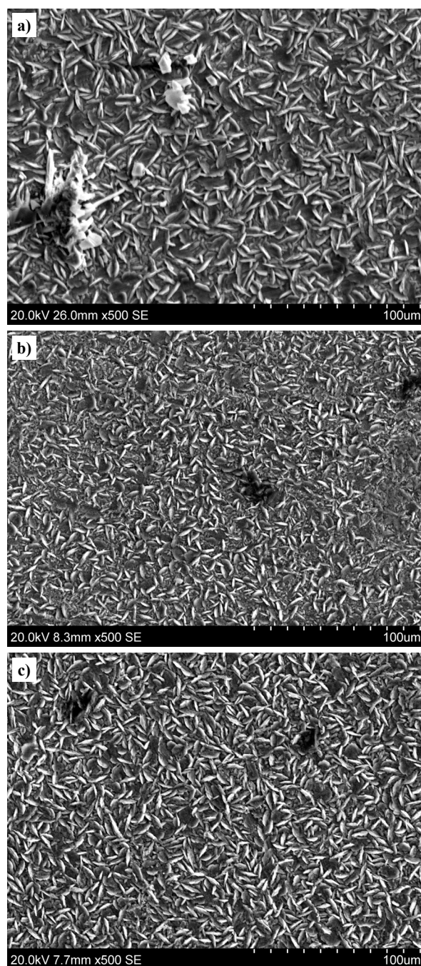
Fig. 2. SEM images of the phosphated (during 10 min.) samples obtained on the nitrided substrate containing layer of nitrides with a thickness of 2 \mu\text{m} (a), 8 \mu\text{m} (b) and 16 \mu\text{m} (c)
