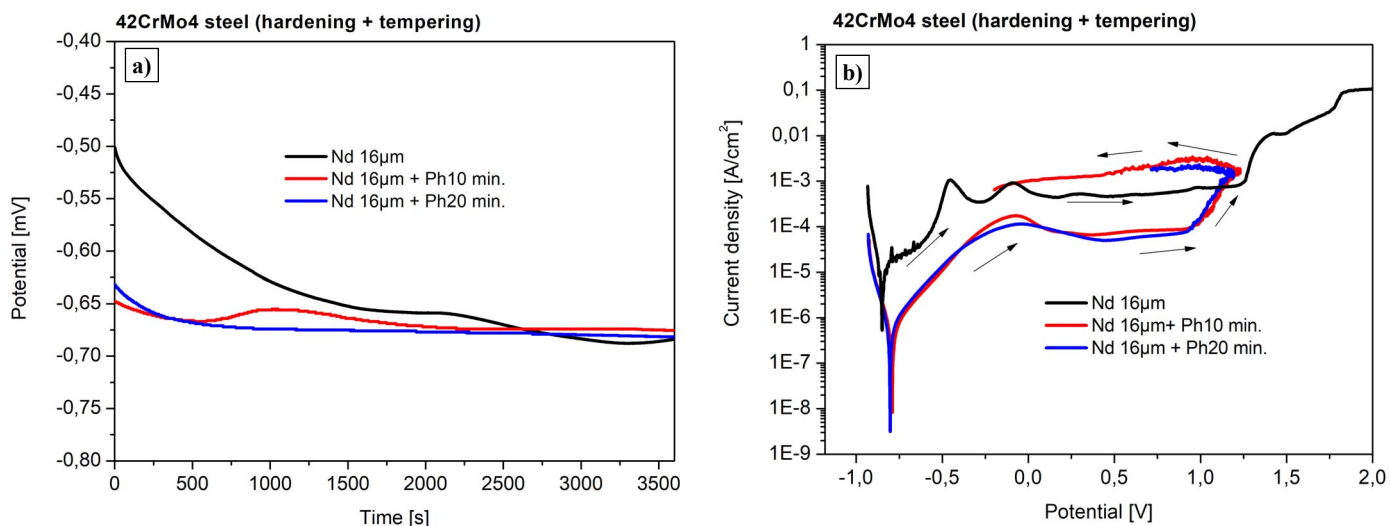
Fig. 6. A course of an open circuit potential a) and polarization curves b) determined after 1 hour of immersion in 0,5 M NaCl for samples of 42CrMo4 nitrided steel (nitrided layer 16 μm) and after 10 min. and 20 min. of phosphating
