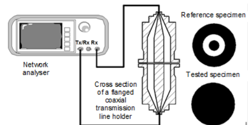
Fig. 29. Measurement test setup for a method complying with ASTM D4935.
