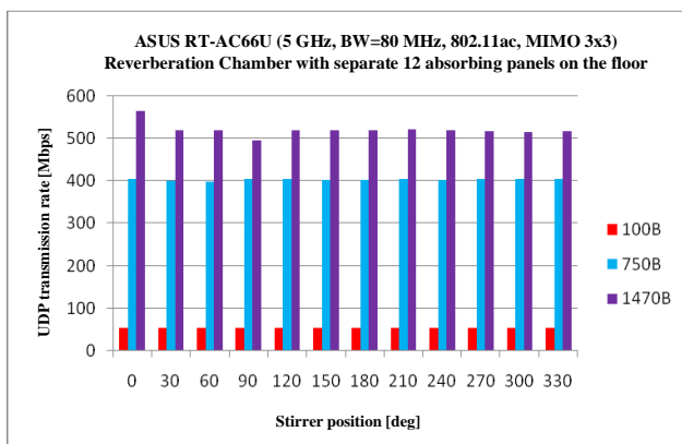
Fig. 20. UDP data transmission rate R_{UDP} measured for ASUS RT-AC66U routers as a function of the stirrer position for separate installation of 12 absorbing panels on RC's floor
