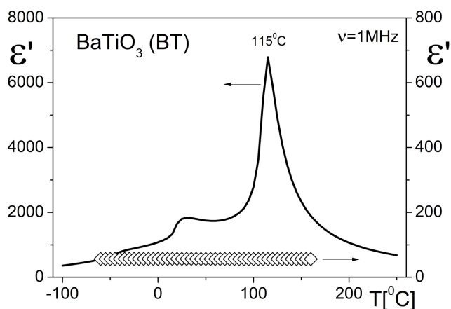
Fig. 6. The temperature dependence of the real part of the dielectric permittivity for the BT samples obtained by the mechanochemical methods (right Y axis) and subjected to subsequent heat treatment (left Y axis)
