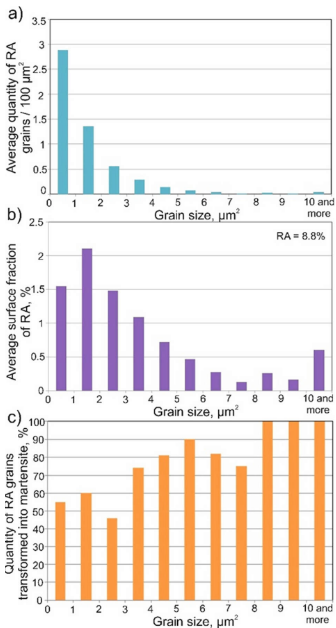
Fig. 8. Statistical evaluation of RA parameters at -20^{\circ}\text{C} : a) average quantity of RA grains per 100\ \mu\text{m}^2 ; b) average surface fraction of RA; c) quantity of retained austenite grains transformed into martensite
