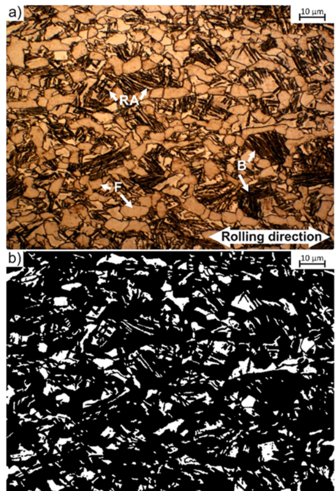
Fig. 4. Initial microstructure of the investigated steel: a) optical micrograph; b) binary map of retained austenite (marked as white)
