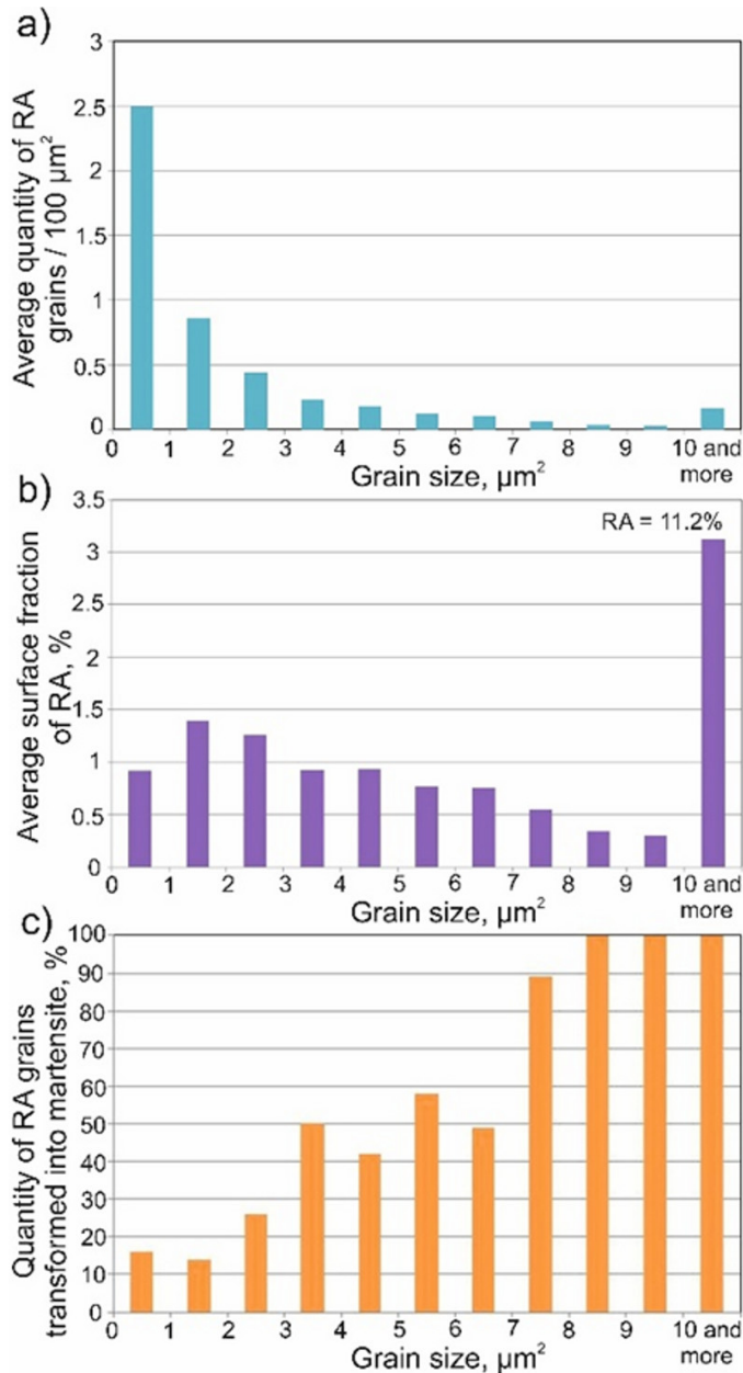
Fig. 10. Statistical evaluation of RA parameters at 20°C: a) average quantity of RA grains per 100 μm 2 ; b) average surface fraction of RA; c) quantity of retained austenite grains transformed into martensite
