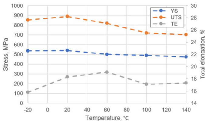
Fig. 3. Changes in mechanical properties as a function of deformation temperature
