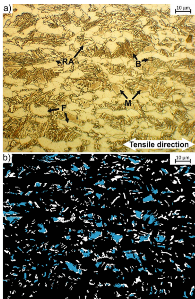
Fig. 7. Microstructure of the investigated steel deformed at -20^\circ\text{C} : a) optical micrograph, b) binary map of retained austenite (white) and martensite (blue)
