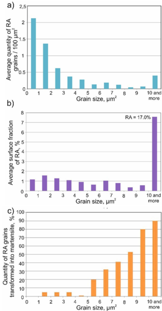
Fig. 12. Statistical evaluation of RA parameters at 100°C: a) average quantity of RA grains per 100 μm 2 ; b) average surface fraction of RA; c) quantity of retained austenite grains transformed into martensite
