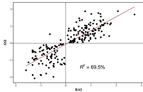
Fig. 12. Scatter plot of standardized streamflow index ( SSI ) and rainfall anomaly index ( RAI ) in monthly during 1999–2018; source: own study
