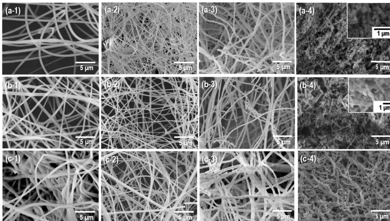
Fig. 2. SEM images of the synthesized Nd-Fe-B materials with different PVP concentrations at each step (as-spun, calcination, reduction, and washing): (a1-4) 3.15 wt%, (b1-4) 3.75 wt%, and (c1-4) 4.35 wt%
