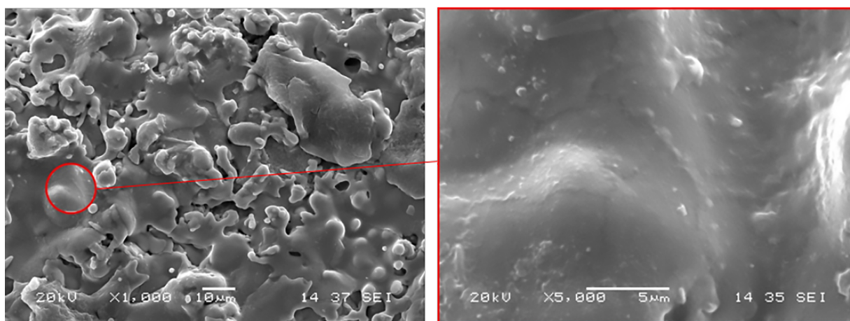
Fig. 2. SEM images of anodized Ti-6Al-7Nb specimens in 1M H2SO4 at 100 V
