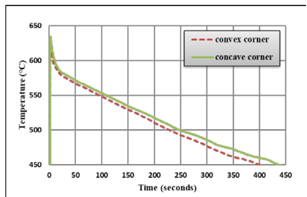
Fig. 12. Thermal profiles at corners of cast part during cooling
