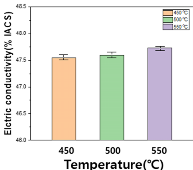
Fig. 5. Electric conductivity of as-extruded Al-2Zn-1Cu-0.5Mg-0.5RE alloy on different temperature at 450, 500 and 550°C
