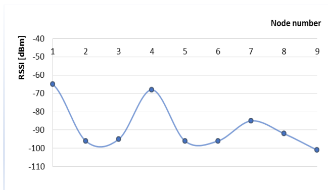
Fig. 14. RSSI versus node number, TX Power=4
