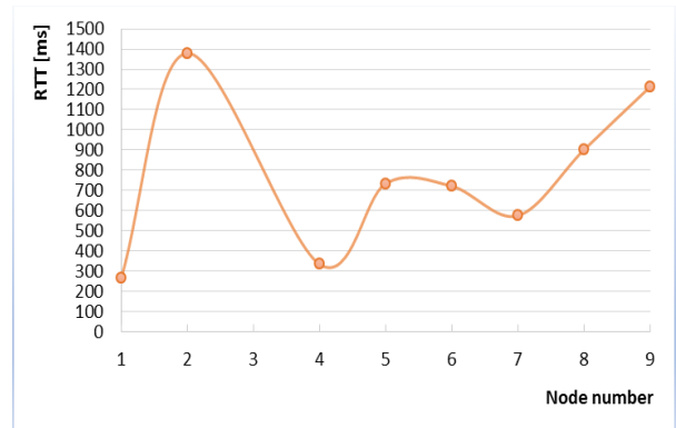
Fig. 12. RTT versus node number, TX Power=3
