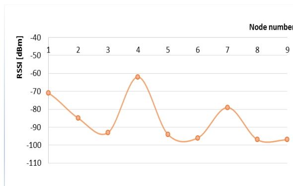
Fig. 17. RSSI versus node number, TX Power = 7
