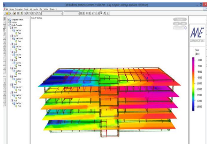
Fig. 7. The result of the radio coverage simulation in P3 building for the Motley-Keenan model, the chosen transmitter is the node 1 (2nd floor - room No. 308) [23]
