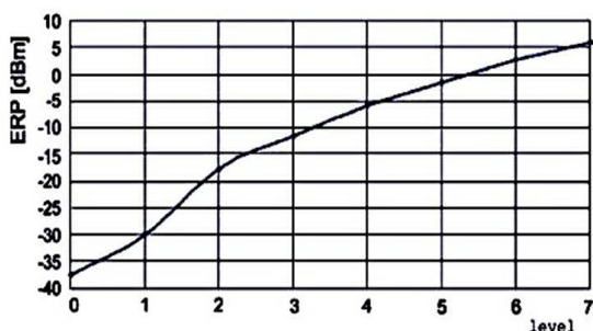
Fig. 4. Effective radiated power (ERP) vs. level in the set TX Power(level) function. TR-72D(A), 868 MHz band, channels 0 to 67[17]
