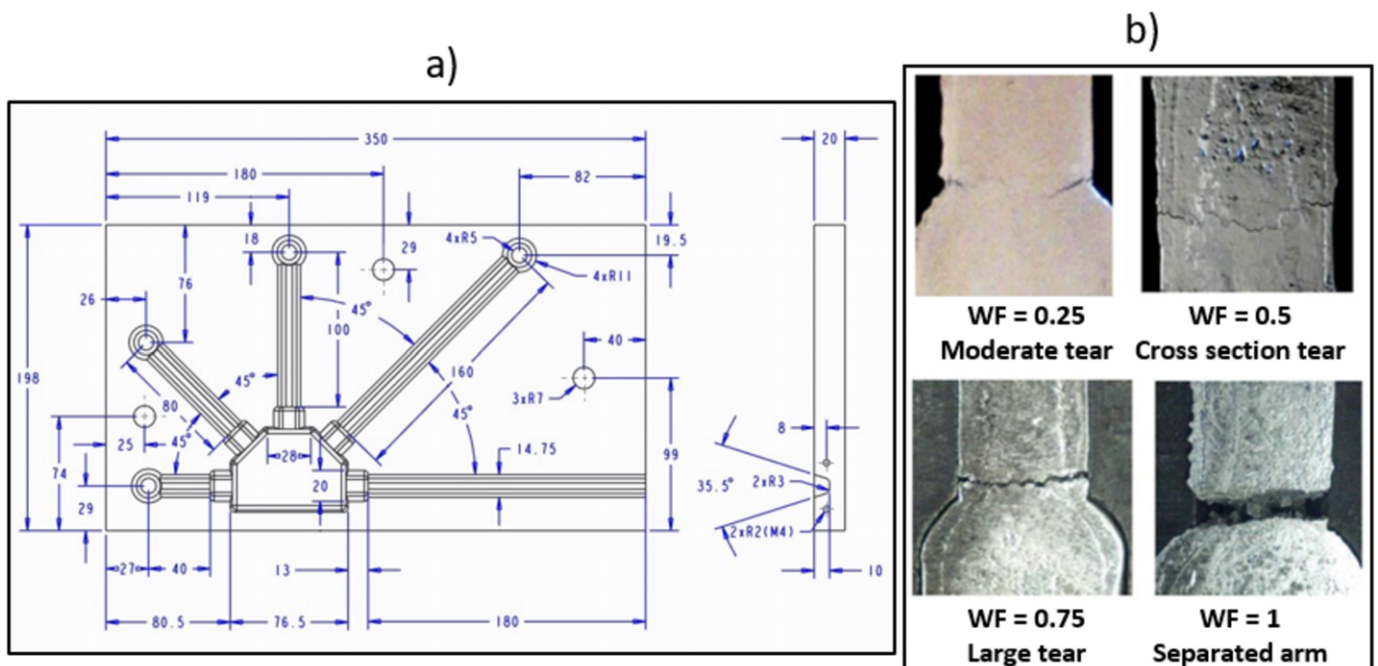
Fig. 9. Hot tearing index: (a) schematic mold; (b) weighting factor categories
