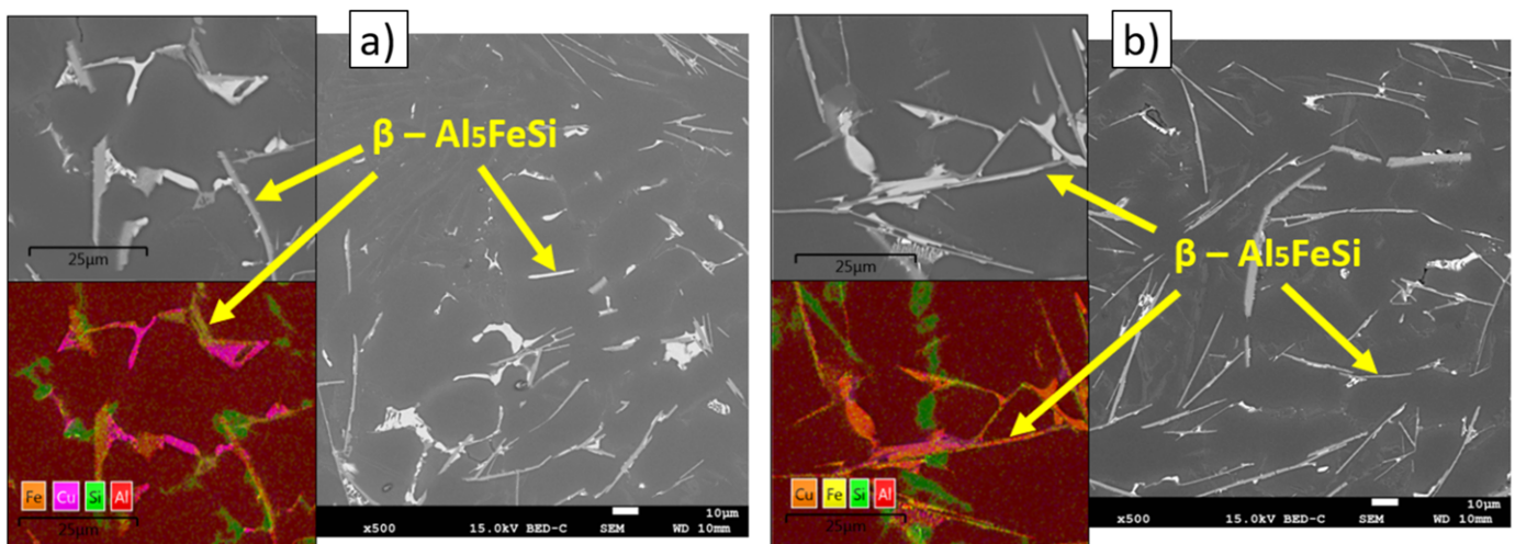
Fig. 5. Iron phases in microstructure after artificial ageing, SEM: (a) 20 – 80 alloy; (b) 90 – 10 alloy
